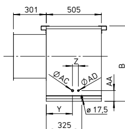
Refrigerant connection side
