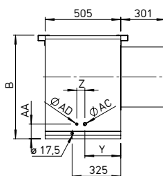
Refrigerant connection side
