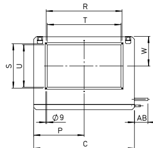
Unit connection side
