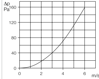
Pressure loss KLF G4 1) Pure state
