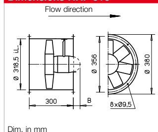
Dimensions HRF 315
