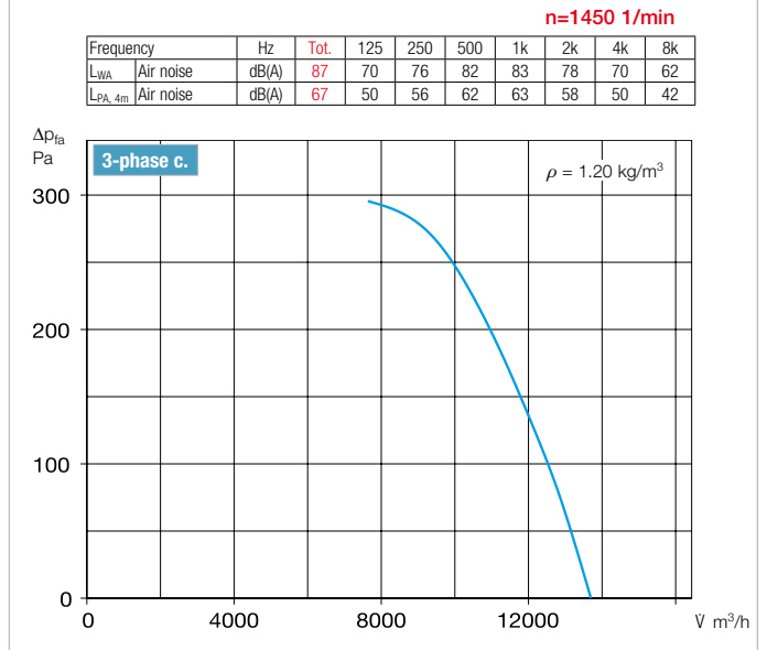
Performance curve VAR 630/6
