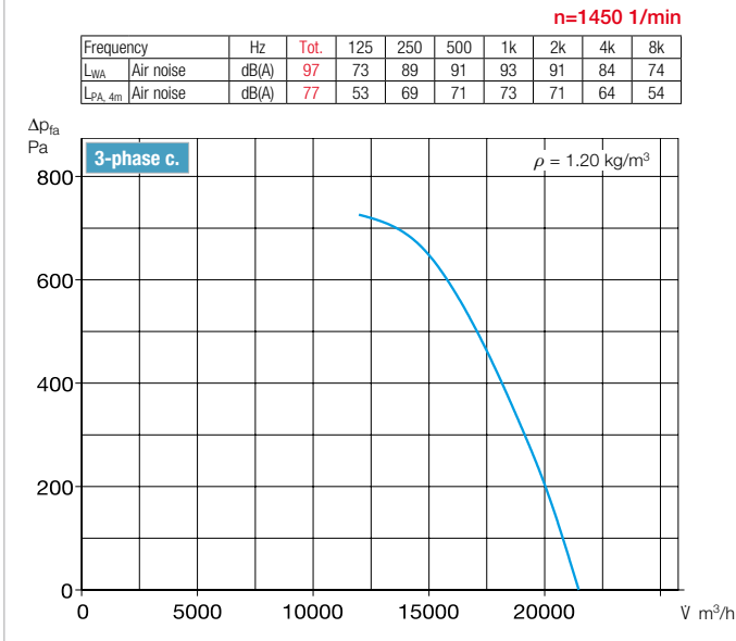
Performance curve VAR 630/4
