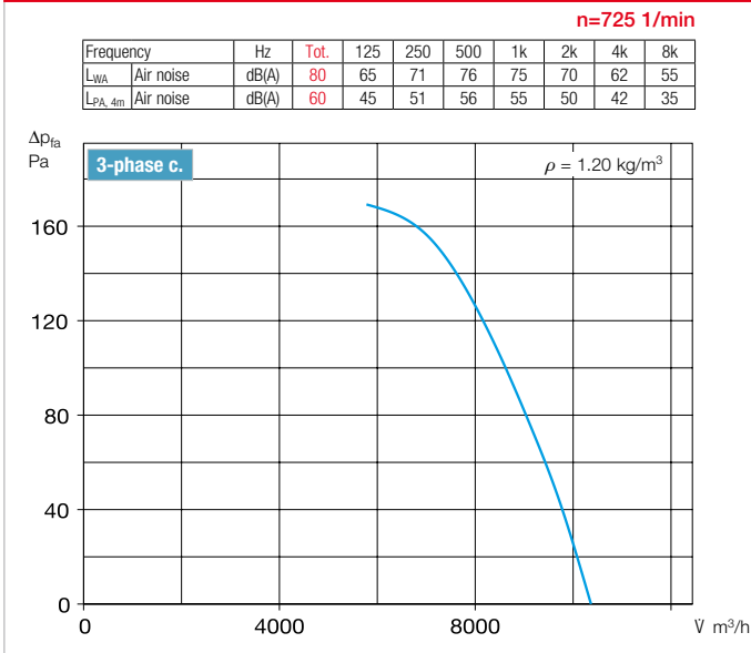
Performance curve VAR 630/8
