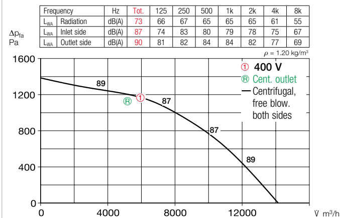
Performance curves GBD 630/4 T120
