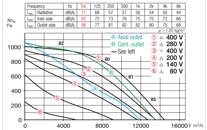
Performance curves GBD 630/4/4
