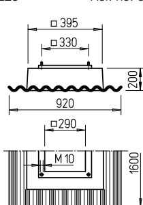
Base silencer, hinged SSD 225
