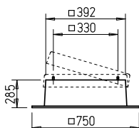
Flat roof base, hinged FDS 225
