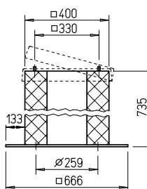
Base silencer, hinged SSD 225
