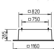
Flat roof base FDS 560
