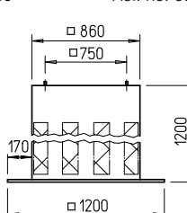
Base silencer SSD 560
