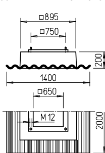
Base silencer SSD 630
