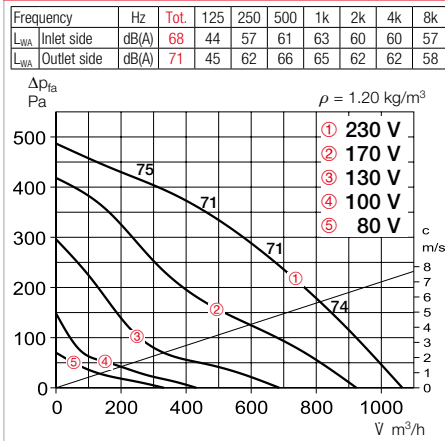
Performance curves RDW 200/2
