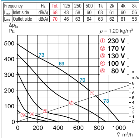
Performance curves VDW 200/2
