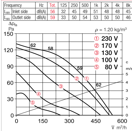
Performance curves RDW 200/4
