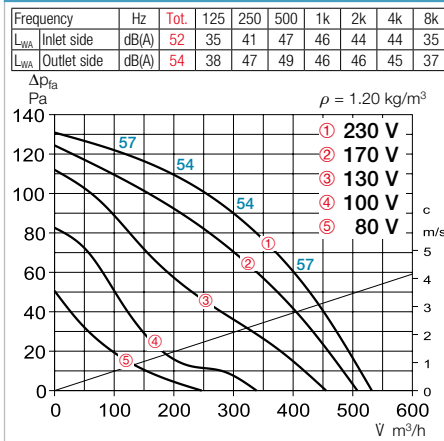
Performance curves VDW 200/4
