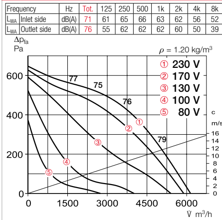
Performance curves RDW 400/4
