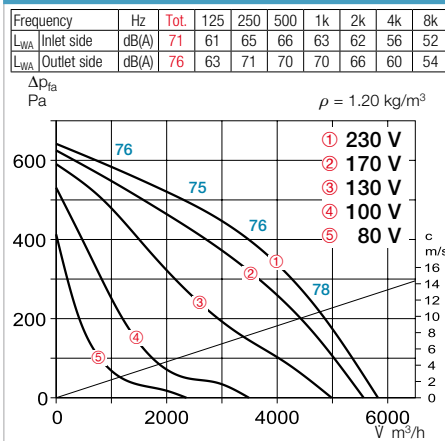
Performance curves VDW 400/4
