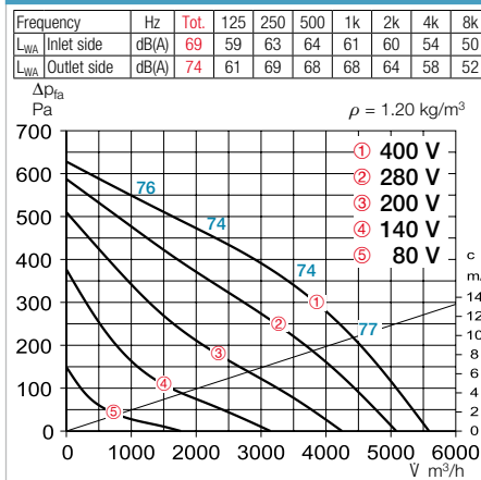
Performance curves VDD 400/4
