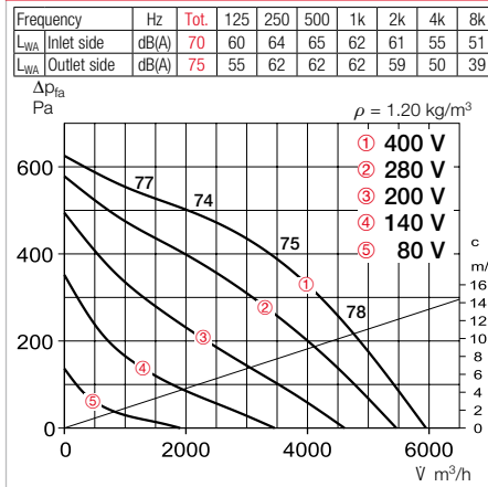
Performance curves RDD 400/4
