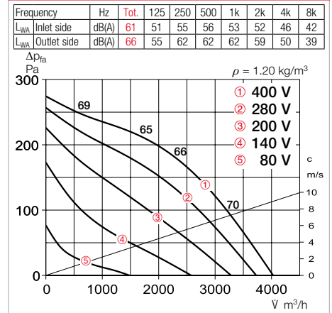
Performance curves RDD 400/6
