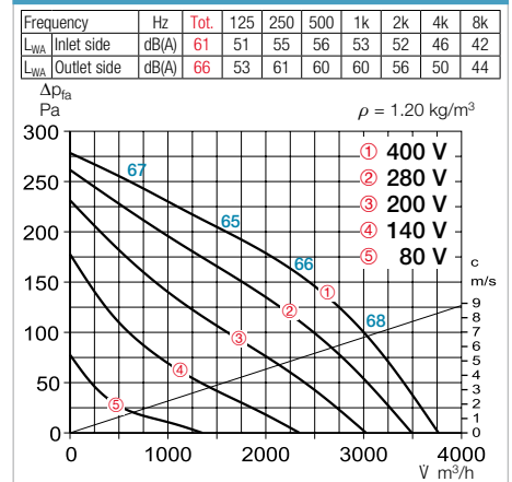
Performance curves VDD 400/6
