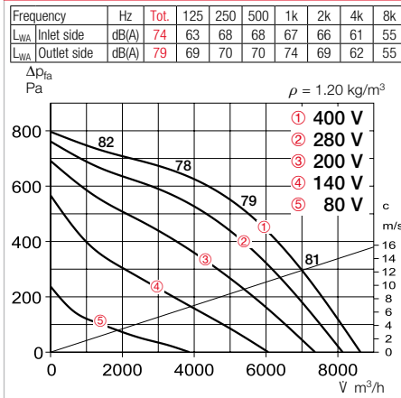
Performance curves RDD 450/4
