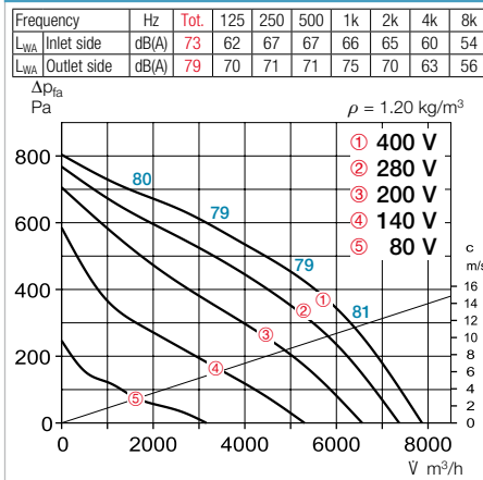
Performance curves VDD 450/4
