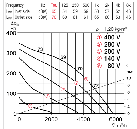
Performance curves RDD 450/6
