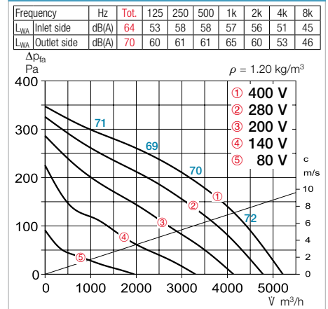
Performance curves VDD 450/6
