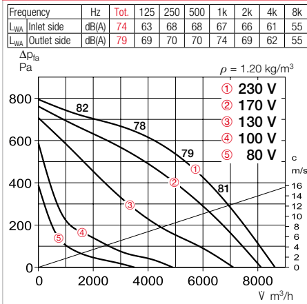
Performance curves RDW 450/4
