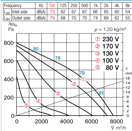
Performance curves VDW 450/4
