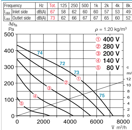
Performance curves VDD 500/6
