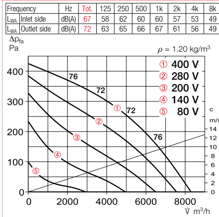
Performance curves RDD 500/6
