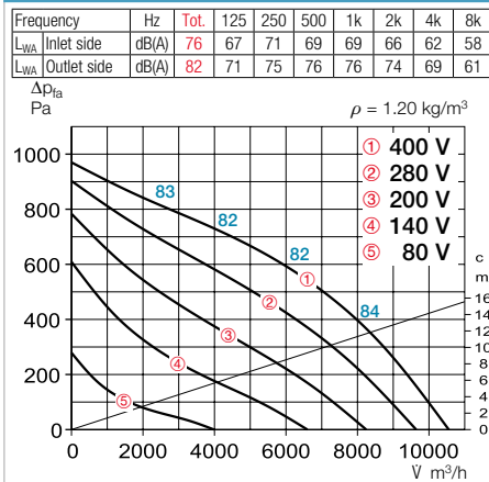
Performance curves VDD 500/4
