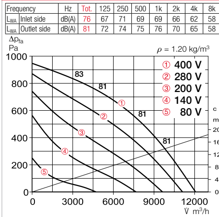
Performance curves RDD 500/4
