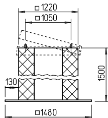
Base silencer SSD 710
