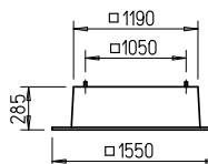
Flat roof base FDS 710
