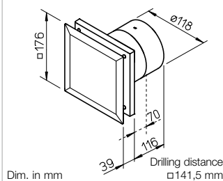
Dimensions M1/120
