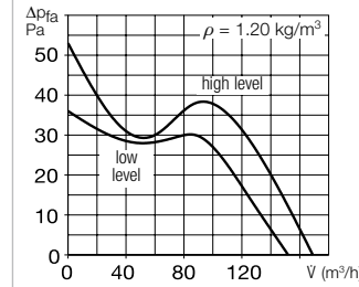
Performance curve M1/120
