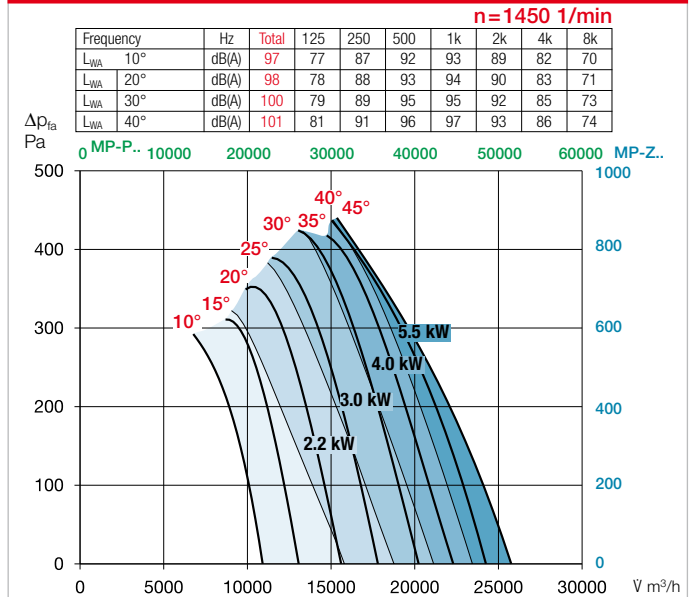
Performance curves AMD / B AMD 630/4
