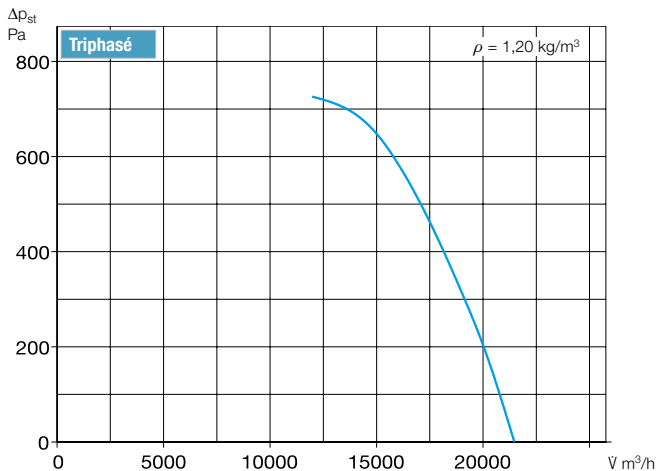
Courbe de performances VAR 630/8
