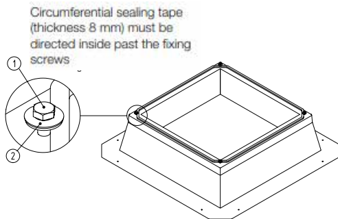
Fig. 2: Flat roof base FDS/FDS-B without hinged cover
