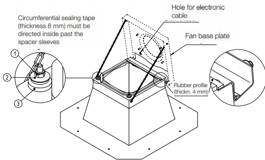
Fig. 1: Flat roof base FDS with hinged cover
