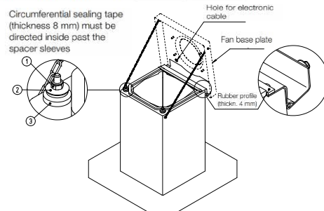
Fig. 3: Base attenuator SSD with hinged cover
