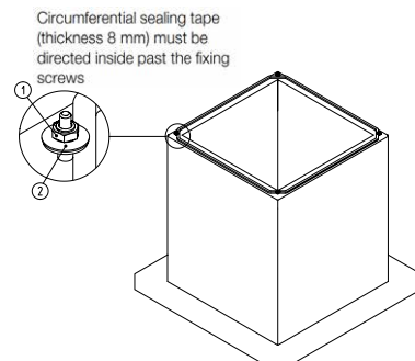
Fig. 4: Base attenuator SSD without hinged cover
