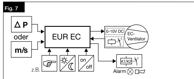
Example 2: Differential pressure control and air velocity control
