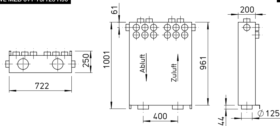
KWL MZB 6+1-75/125 L90
