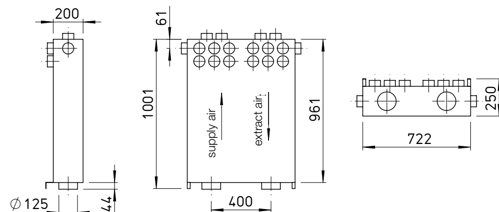
KWL MZB 6+1-75/125 L90
