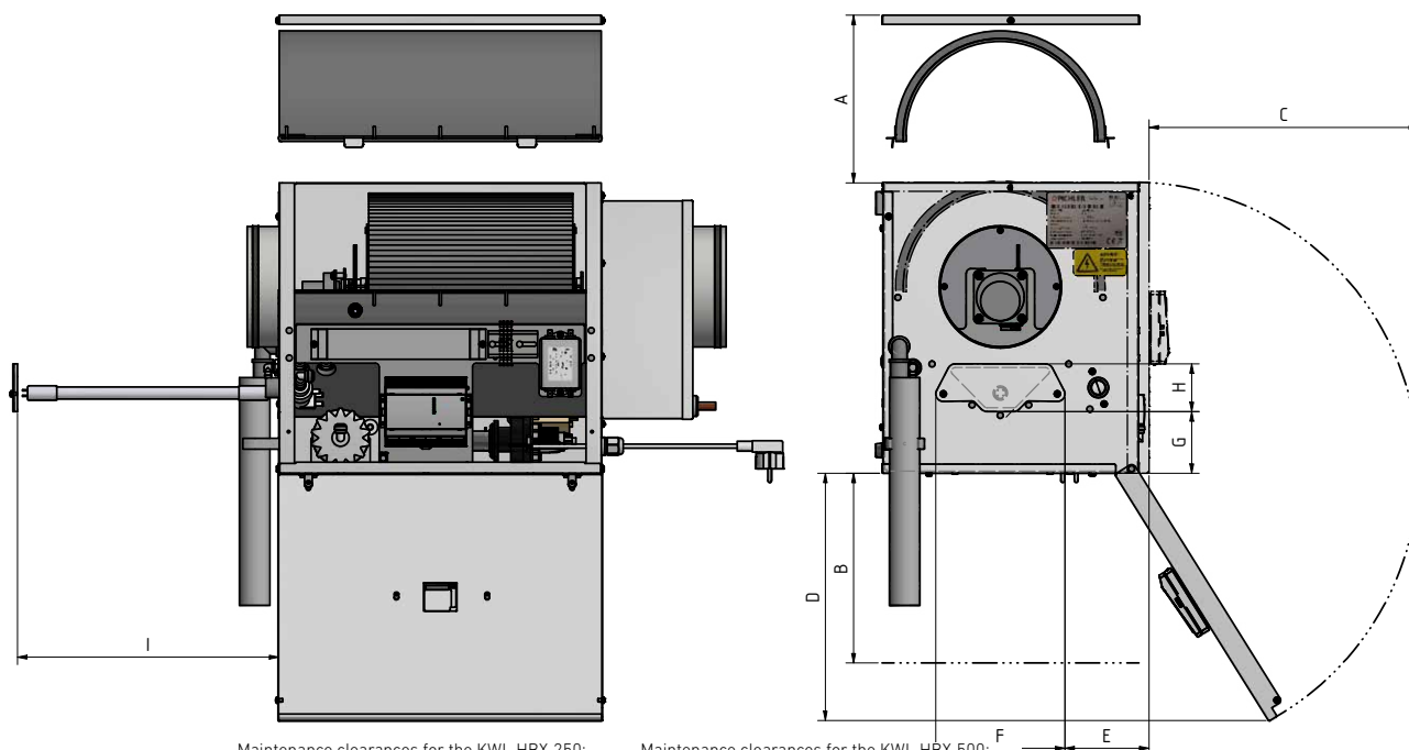
Maintenance clearances for the KWL HBX 250:
