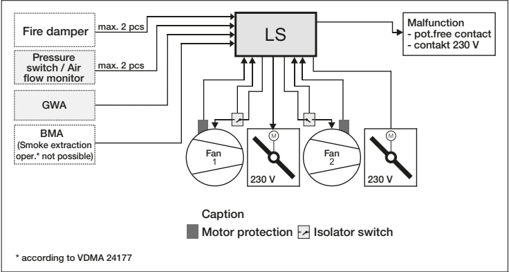
System diagram LS
