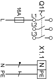
Alimentation 1
