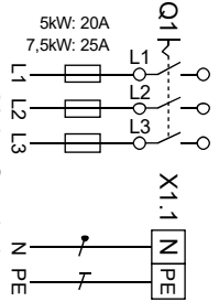
Mains Supply 1
