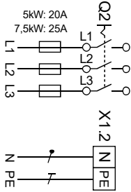
Mains Supply 2
