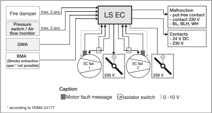
System diagram LS EC
