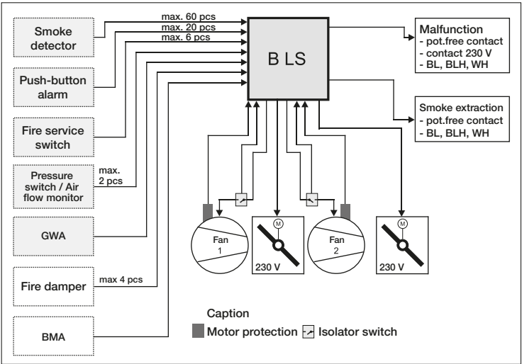
System diagram B LS with smoke ext- raction function
